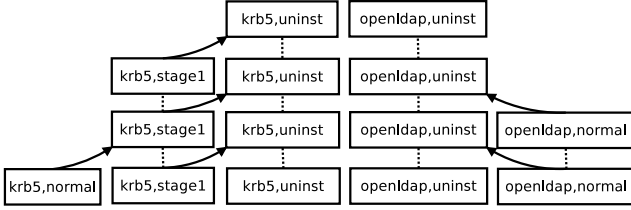
Fig. 3: Reachability graph for the kerberos running example.
