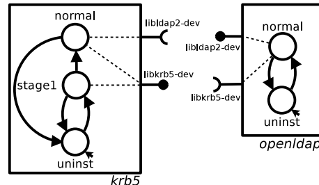
Fig. 2: Representation of the krb5 and openldap components.
