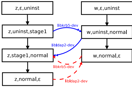
Fig. 5: Abstract plan for the kerberos running example.
