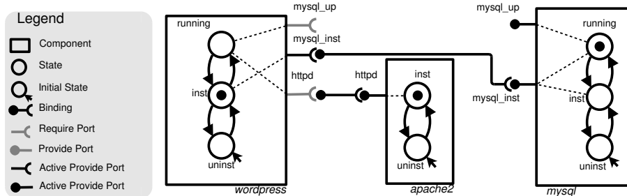
Fig. 1: Wordpress installation in the Aeolus model.
